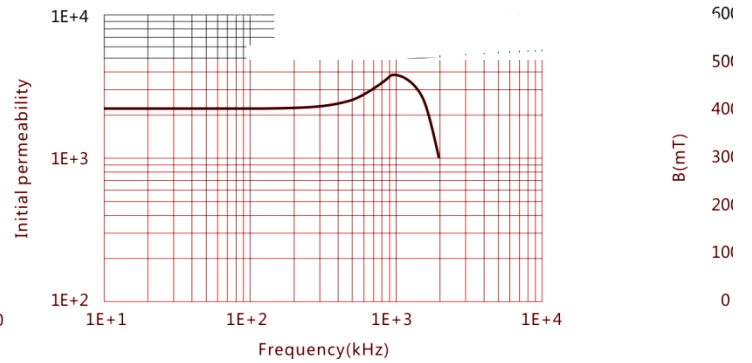
\mu_i -Frequency
